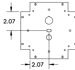
90° X Bracket
