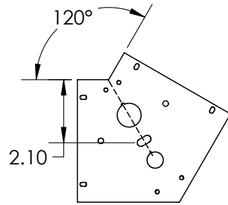
120° Bracket
