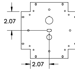
90° X Bracket
