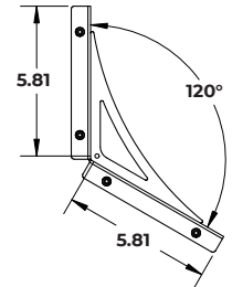
120° Bracket
